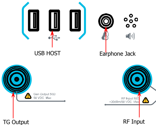
Figure 1-6 Front Panel Connector
