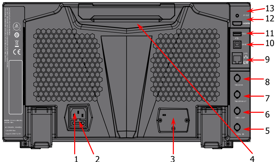
Figure 1-8 Rear Panel
