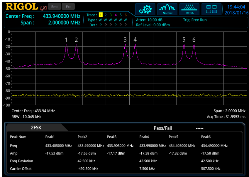
Figure 3-8 SSC Measurement Interface
